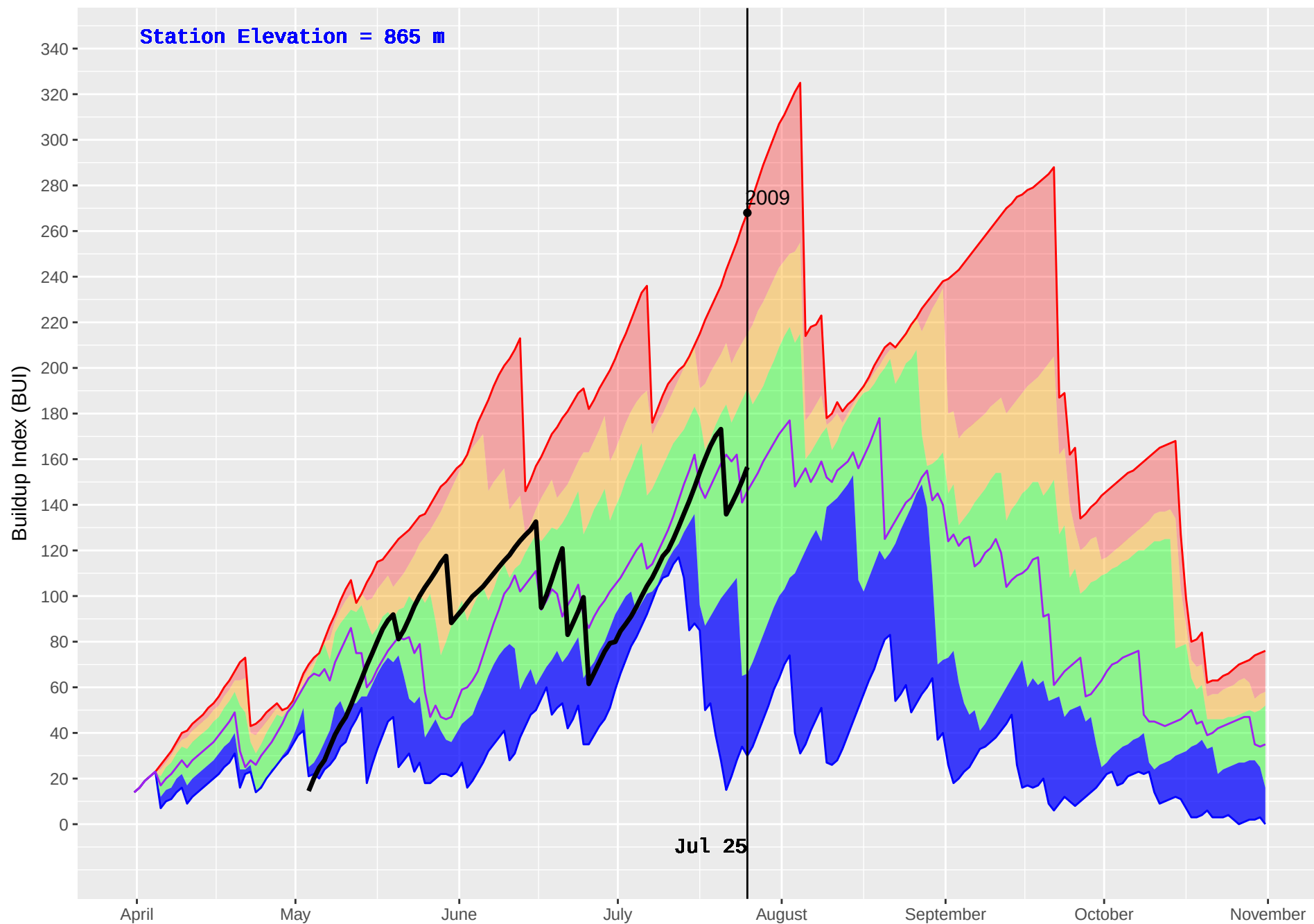
FIVE MILE (1029) : Historical (2008–2016) and Current (2018) Noon Buildup Index (BUI)
